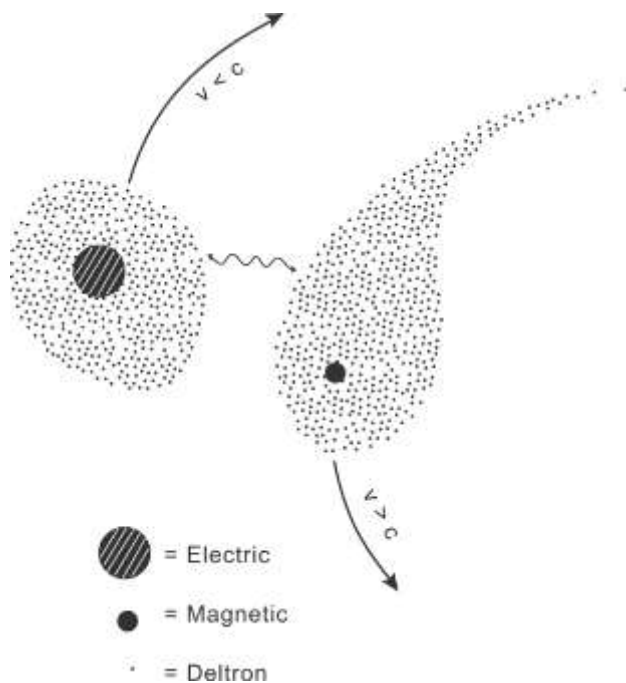
Figure 3. A higher dimensional level of substance, labeled deltrons, falling outside the constraints of relativity theory and able to move at velocities greater than and less than c , acts as a coupling agent between the electric monopole types of substance and the magnetic monopole types of substance to produce both electromagnetic (EM) and magnetoelectric (ME) types of mediator fields exhibiting a special type of “mirror” principle relationship between them.
